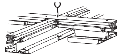
Join of 2 separators
