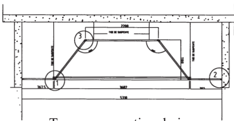
Transverse sectional view
