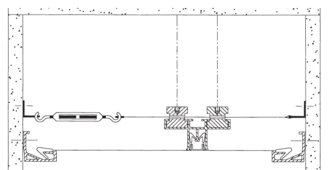
Very high plenum height: the separator is fixed at regular intervals to the ceiling with steel cables and to the wall with stretching devices.
