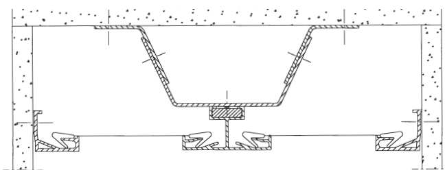
Low plenum height: the separator is fixed to the ceiling
