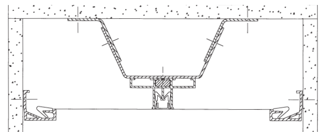
High plenum height: the separator is fixed to the ceiling, at regular intervals, with an adjustable device.
