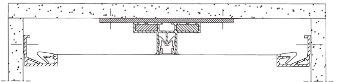
Low plenum height: the separator is fixed to the ceiling
